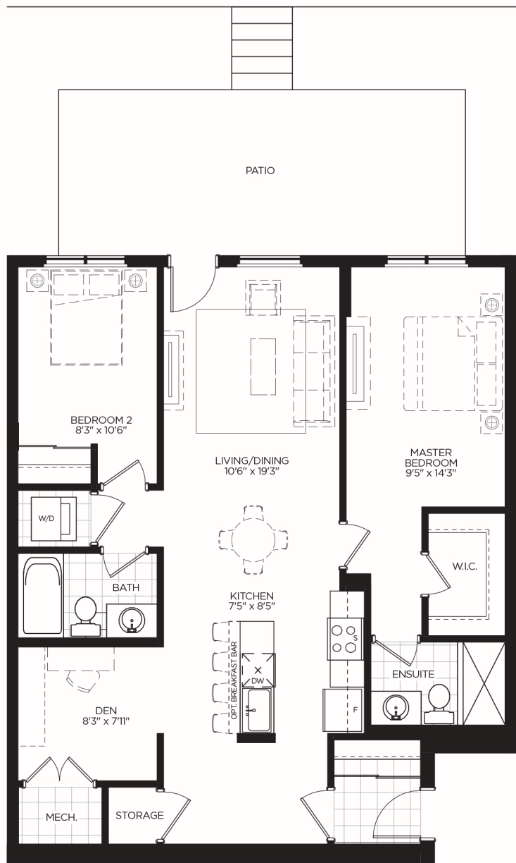
B-LL-INT GARDEN FLOOR
