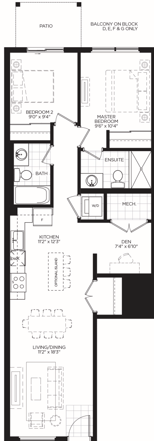
B-GF-INT GROUND FLOOR
