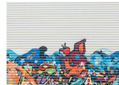
Local Neighbourhood
