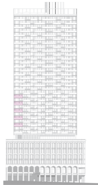
WEST ELEVATION
