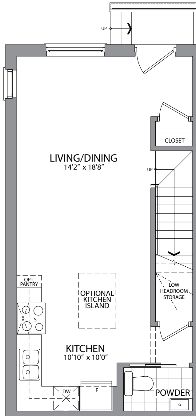
GROUND LEVEL
